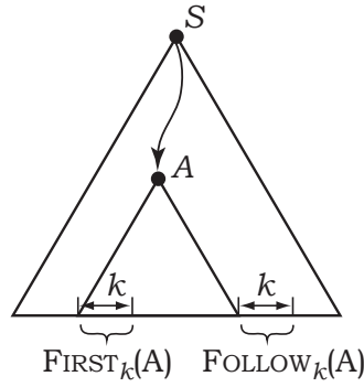
Figure 8.2: Strings in \text{FIRST}_k(A) and in \text{FOLLOW}_k(A) .
